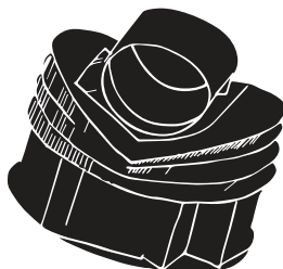
Ariel
