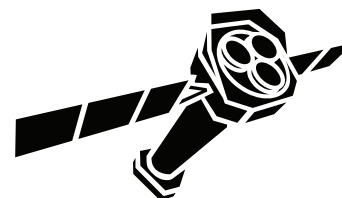
XMM Newton
