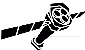
XMM Newton
