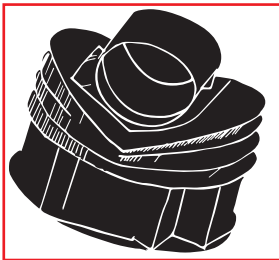
Ariel
